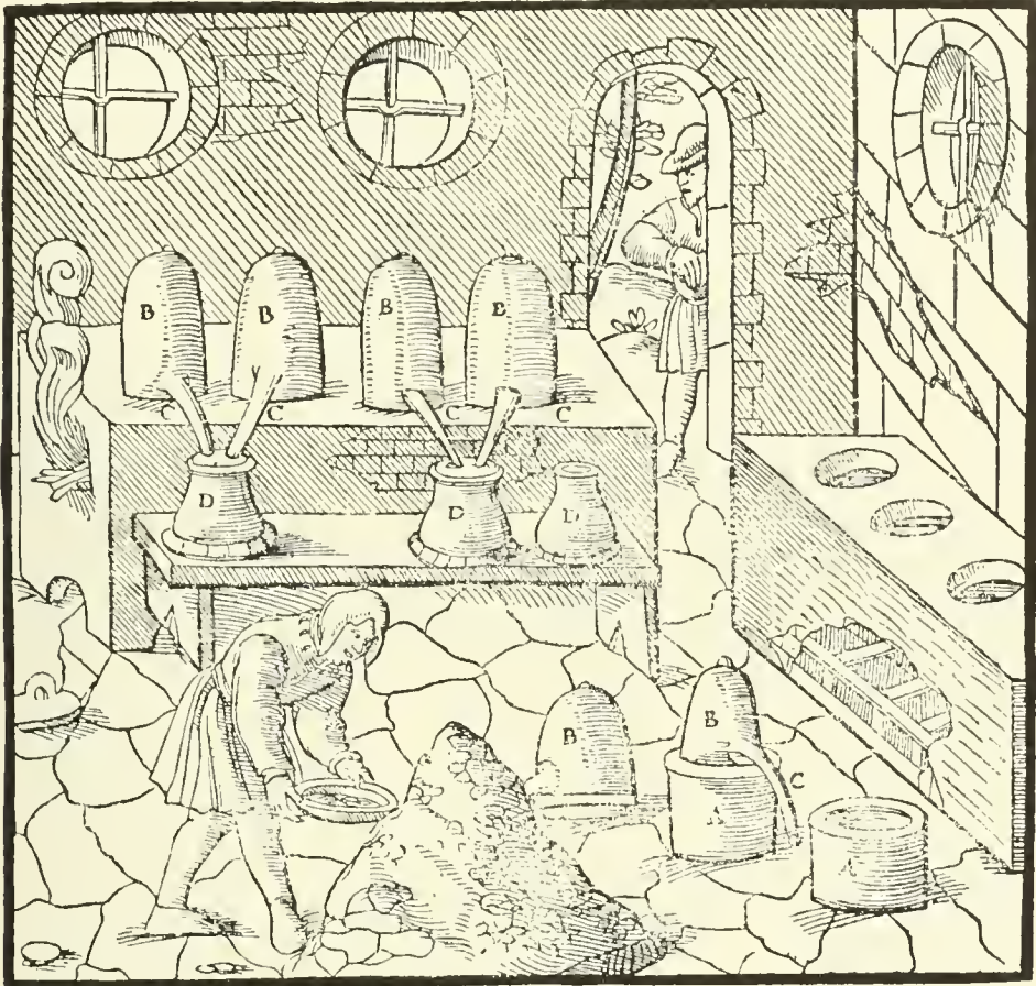
A—POTS. B—OPERCULA. C—NOZZLES. D—GOURD-SHAPED EARTHENWARE VESSELS.
